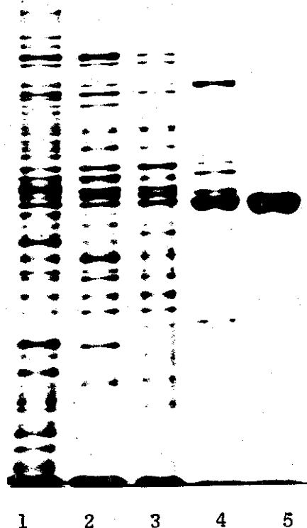
Fig. 1. Purification of GDH(NADPH) 1. Crude Extract; 2. After heating; 3. (NH 4 ) 2 SO 4 precipitate; 4. DEAE-Sepharose eluate; 5. Reactive Blue-Sepharose eluate
